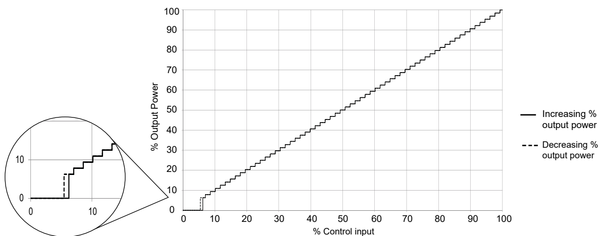
Mode 4: 16 Full cycles switching
