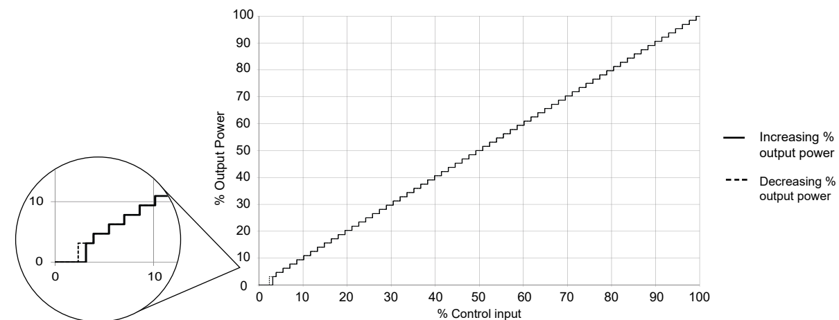
Mode 3: 4 Full cycles switching
