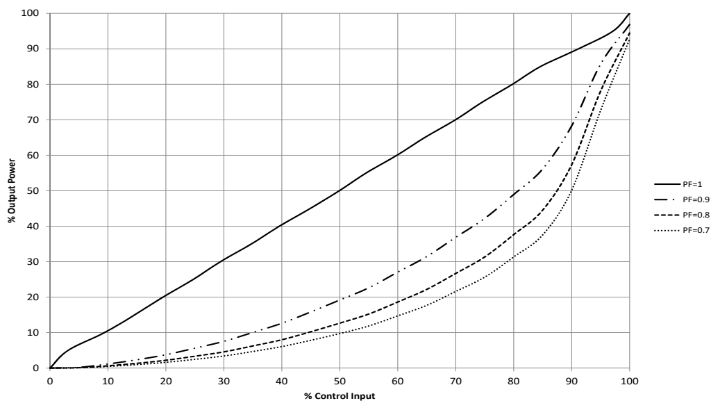
Mode 1: Phase angle switching
